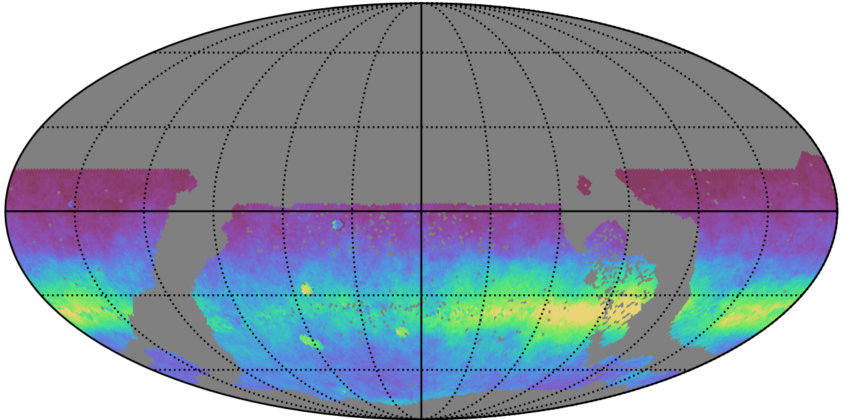
early_ss_template_fpextra3.0_v3.4_10yrs WFD all bands: AngleRms rotSkyPos
