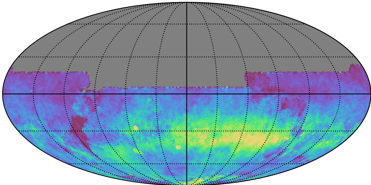
early_ss_template_fpextra3.0_v3.4_10yrs All sky y band: AngleRms rotSkyPos
