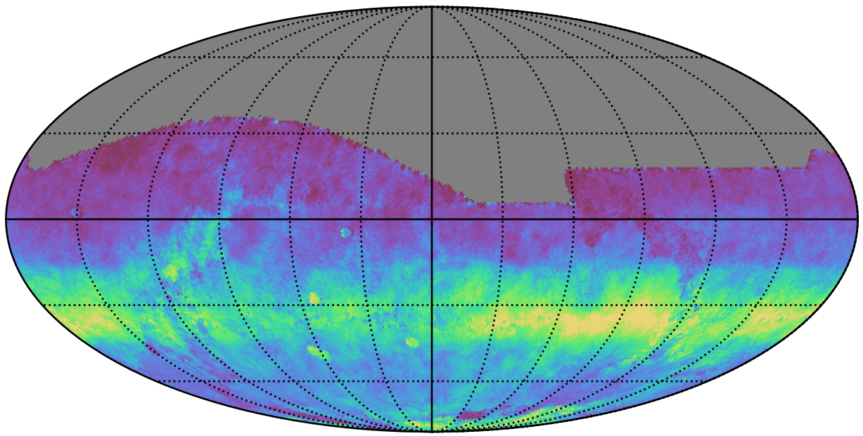
early_ss_template_fpextra3.0_v3.4_10yrs All sky r band: AngleRms rotSkyPos
