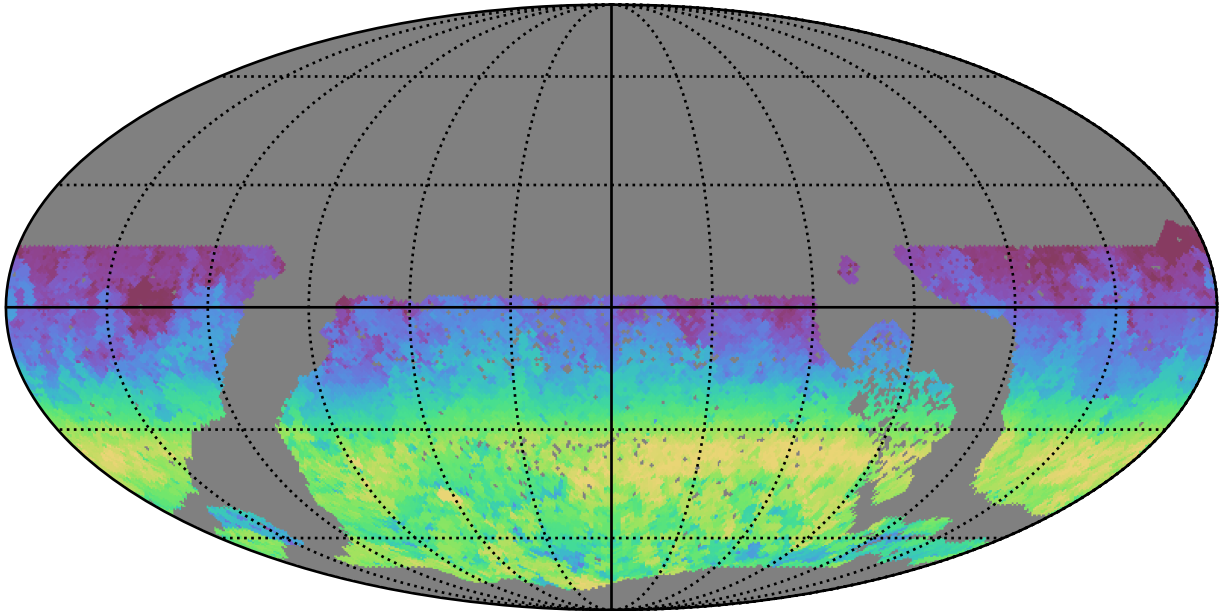
early_ss_template_fpextra3.0_v3.4_10yrs WFD z band: AngleRange rotSkyPos
