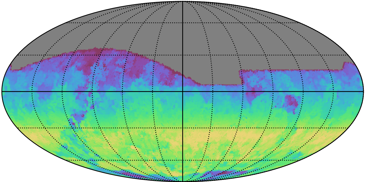
early_ss_template_fpextra3.0_v3.4_10yrs All sky z band: AngleRange rotSkyPos
