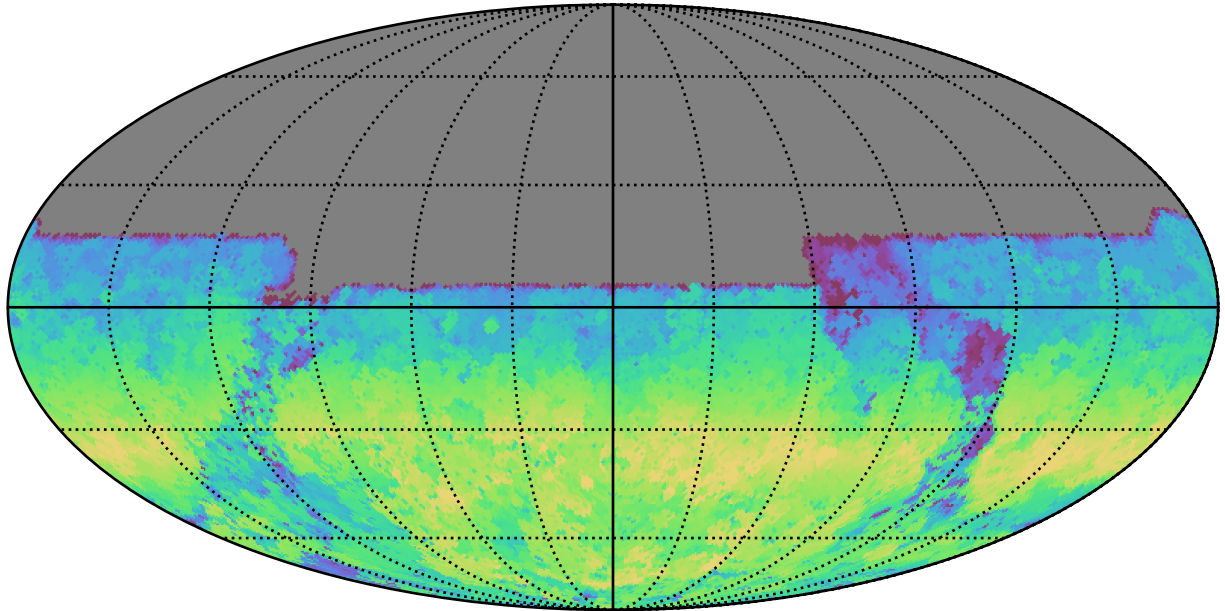
early_ss_template_fpextra3.0_v3.4_10yrs All sky u band: AngleRange rotSkyPos
