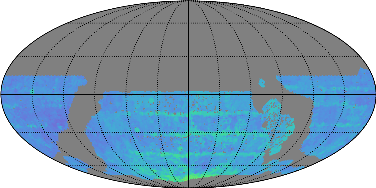
early_ss_template_fpextra3.0_v3.4_10yrs WFD z band: 80thPercentile Season Length
