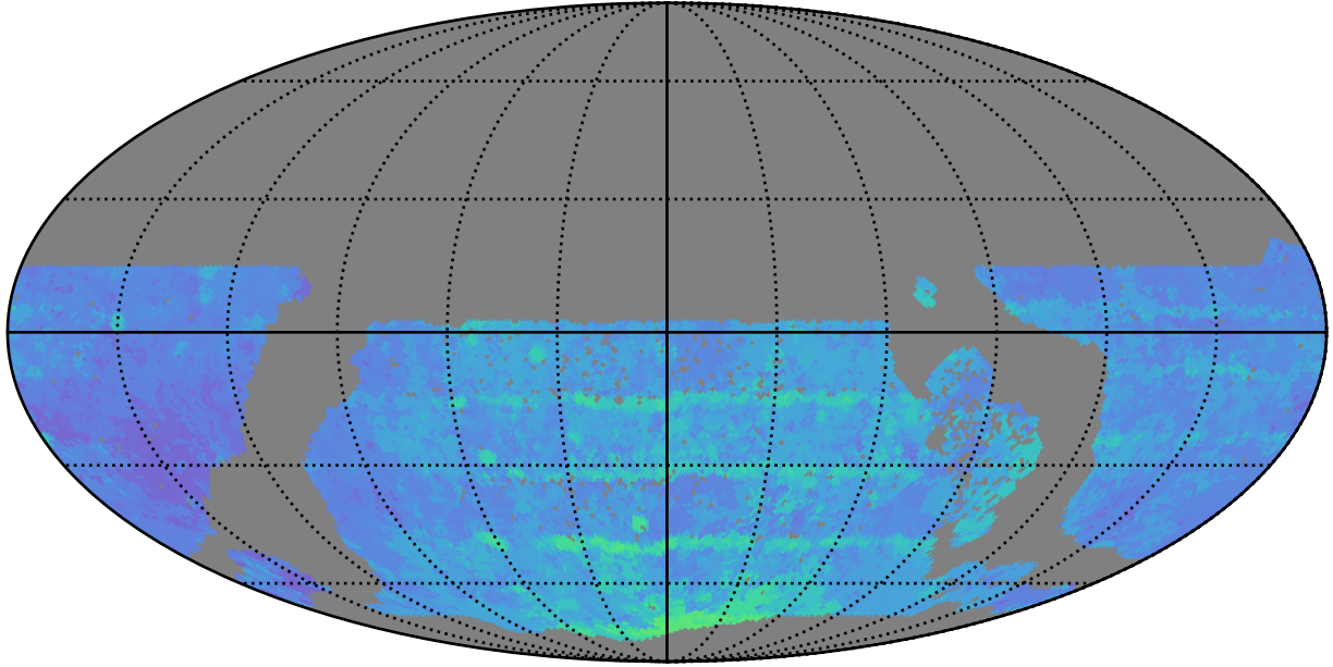
early_ss_template_fpextra3.0_v3.4_10yrs WFD y band: 80thPercentile Season Length
