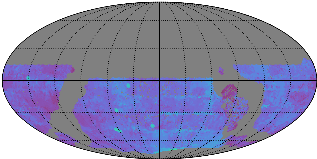
early_ss_template_fpextra3.0_v3.4_10yrs WFD u band: 80thPercentile Season Length
