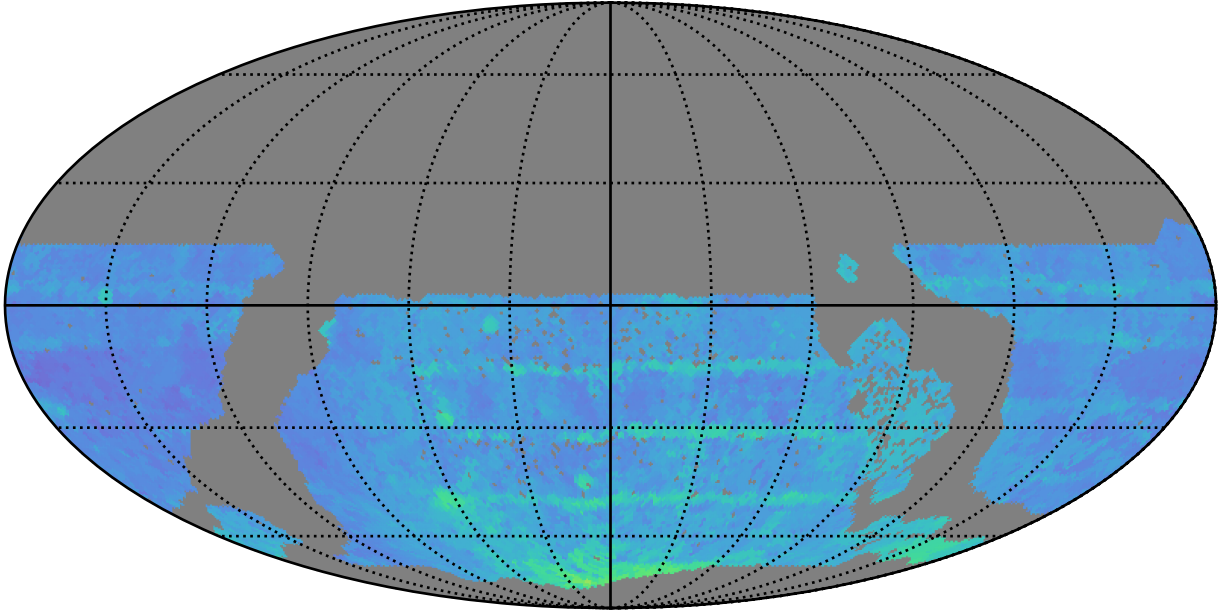
early_ss_template_fpextra3.0_v3.4_10yrs WFD r band: 80thPercentile Season Length
