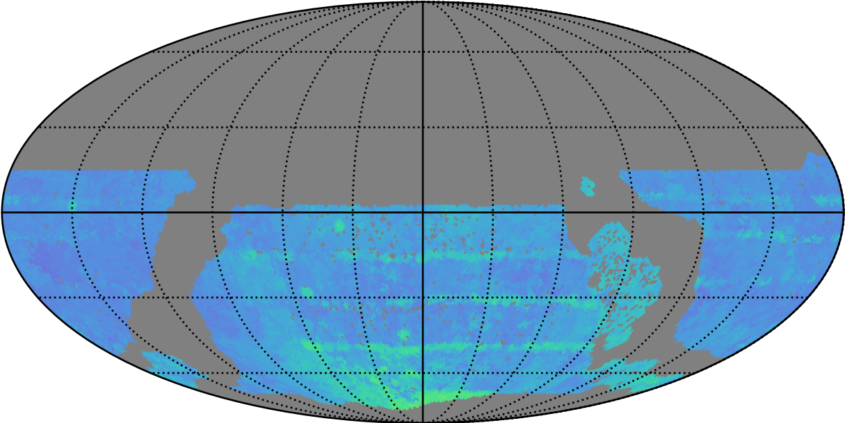
early_ss_template_fpextra3.0_v3.4_10yrs WFD i band: 80thPercentile Season Length
