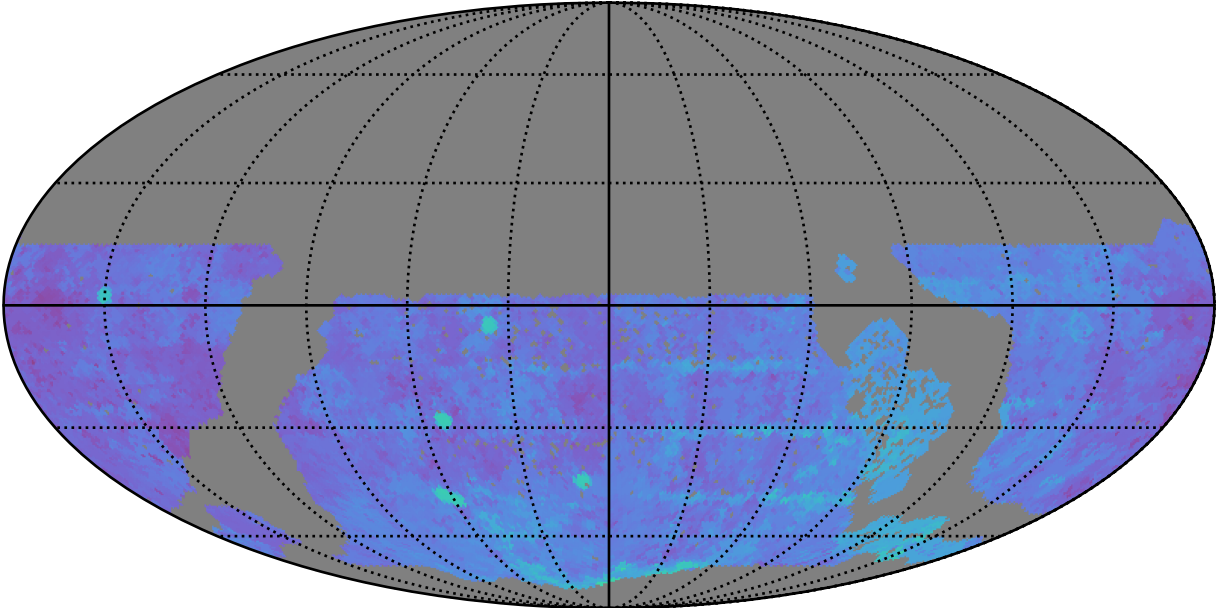
early_ss_template_fpextra3.0_v3.4_10yrs WFD g band: 80thPercentile Season Length
