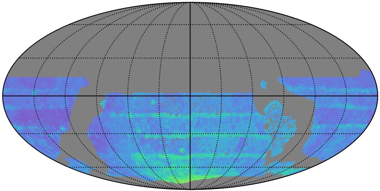
early_ss_template_fpextra3.0_v3.4_10yrs WFD all bands: 80thPercentile Season Length
