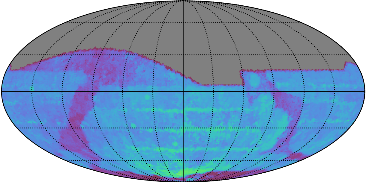
early_ss_template_fpextra3.0_v3.4_10yrs All sky z band: 80thPercentile Season Length
