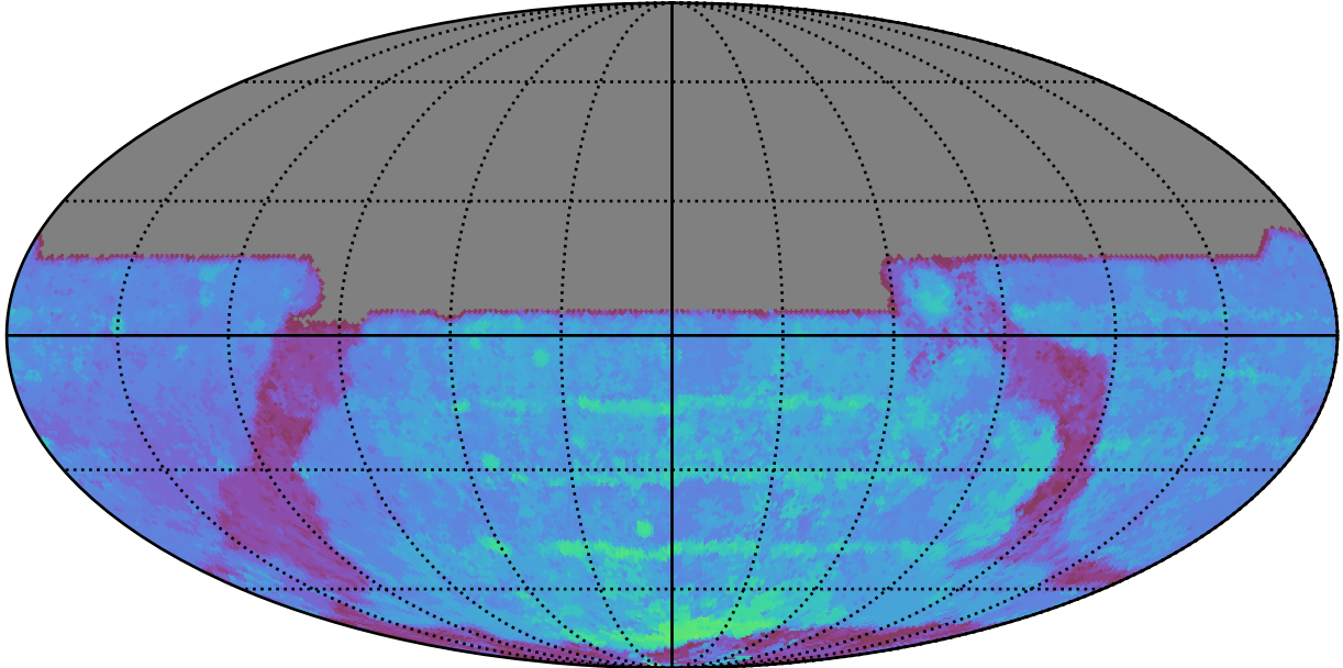
early_ss_template_fpextra3.0_v3.4_10yrs All sky y band: 80thPercentile Season Length
