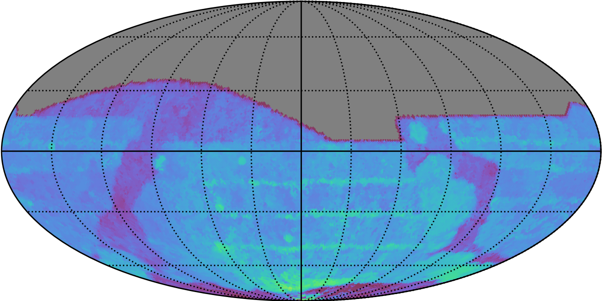
early_ss_template_fpextra3.0_v3.4_10yrs All sky r band: 80thPercentile Season Length
