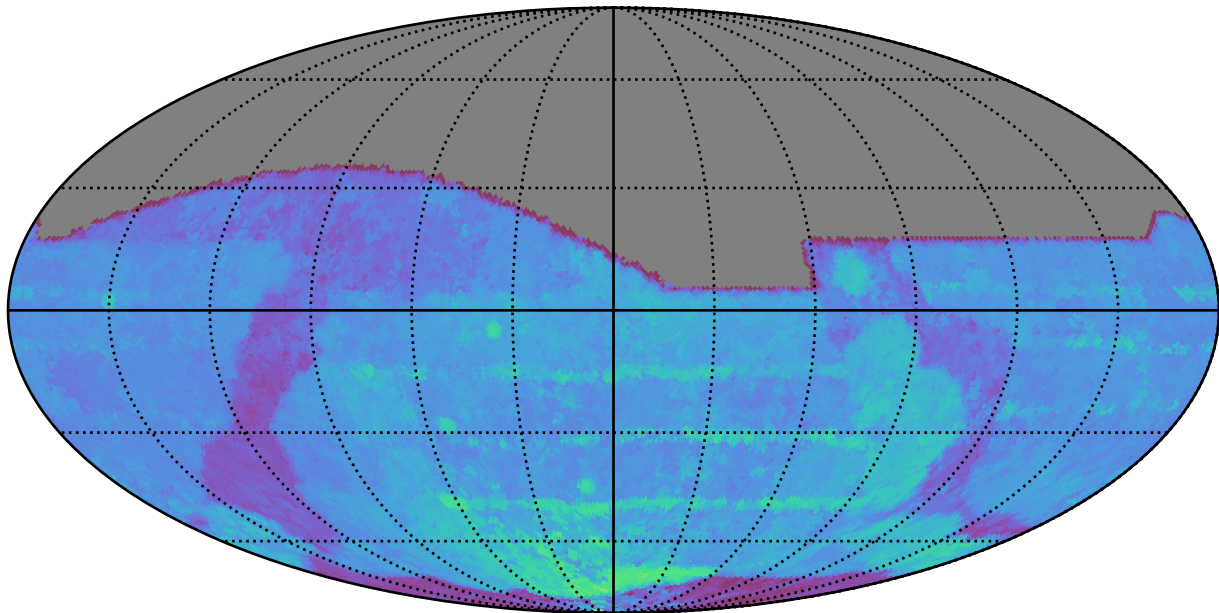
early_ss_template_fpextra3.0_v3.4_10yrs All sky i band: 80thPercentile Season Length
