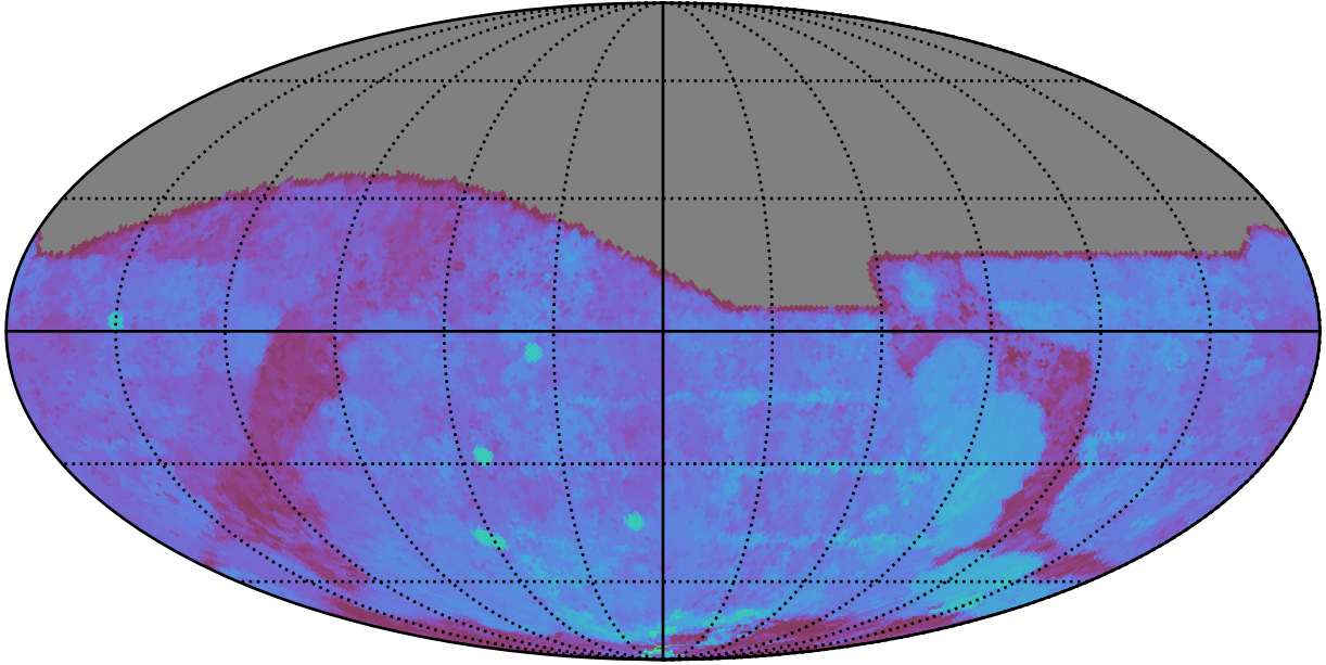
early_ss_template_fpextra3.0_v3.4_10yrs All sky g band: 80thPercentile Season Length
