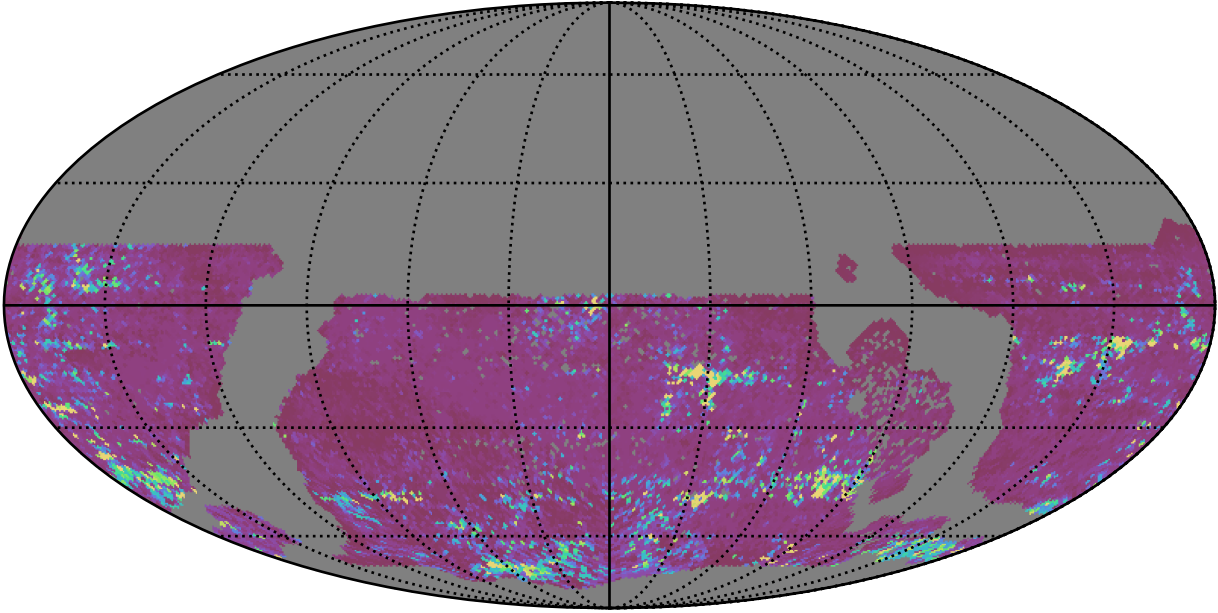
early_ss_template_fpextra3.0_v3.4_10yrs WFD z band: 75th Percentile Intranight Timespan
