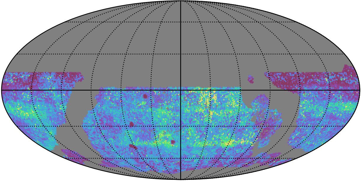
early_ss_template_fpextra3.0_v3.4_10yrs WFD y band: 75th Percentile Intranight Timespan
