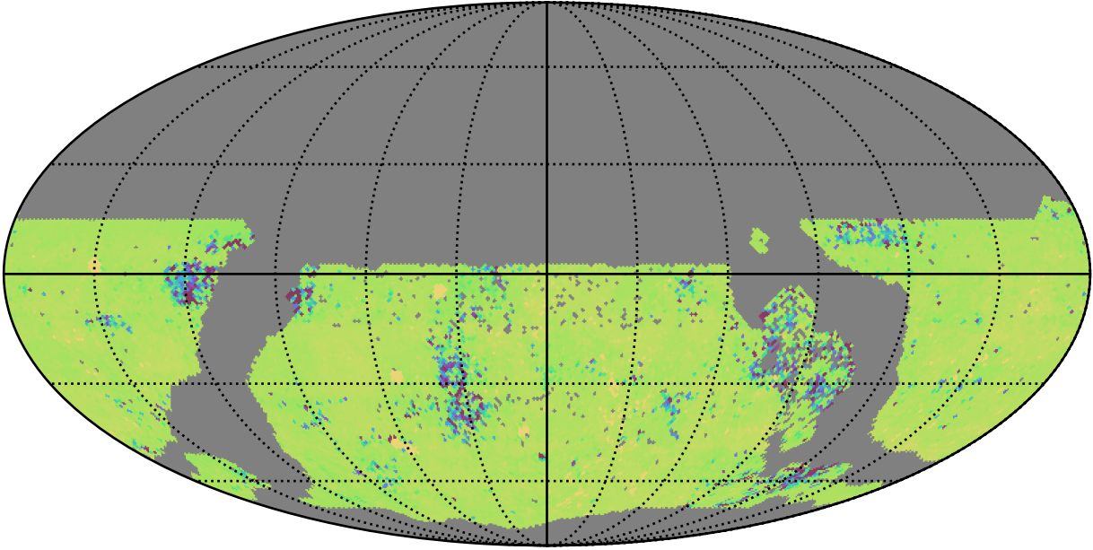
early_ss_template_fpextra3.0_v3.4_10yrs WFD ug bands: 75th Percentile Intranight Timespan
