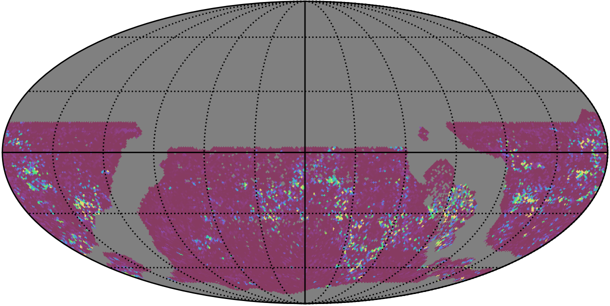
early_ss_template_fpextra3.0_v3.4_10yrs WFD u band: 75th Percentile Intranight Timespan
