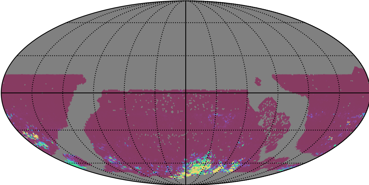
early_ss_template_fpextra3.0_v3.4_10yrs WFD ri bands: 75th Percentile Intranight Timespan
