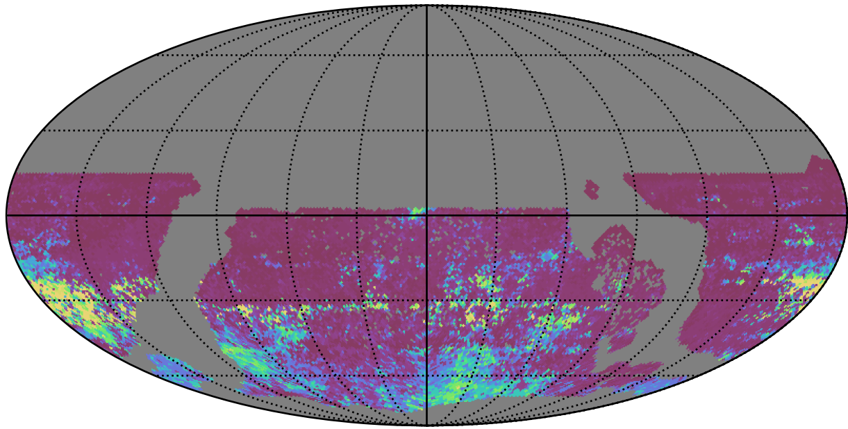
early_ss_template_fpextra3.0_v3.4_10yrs WFD r band: 75th Percentile Intranight Timespan
