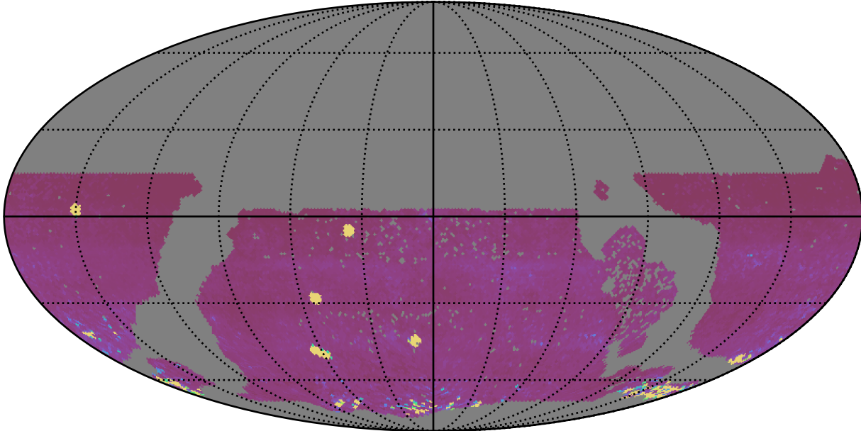
early_ss_template_fpextra3.0_v3.4_10yrs WFD iz bands: 75th Percentile Intranight Timespan
