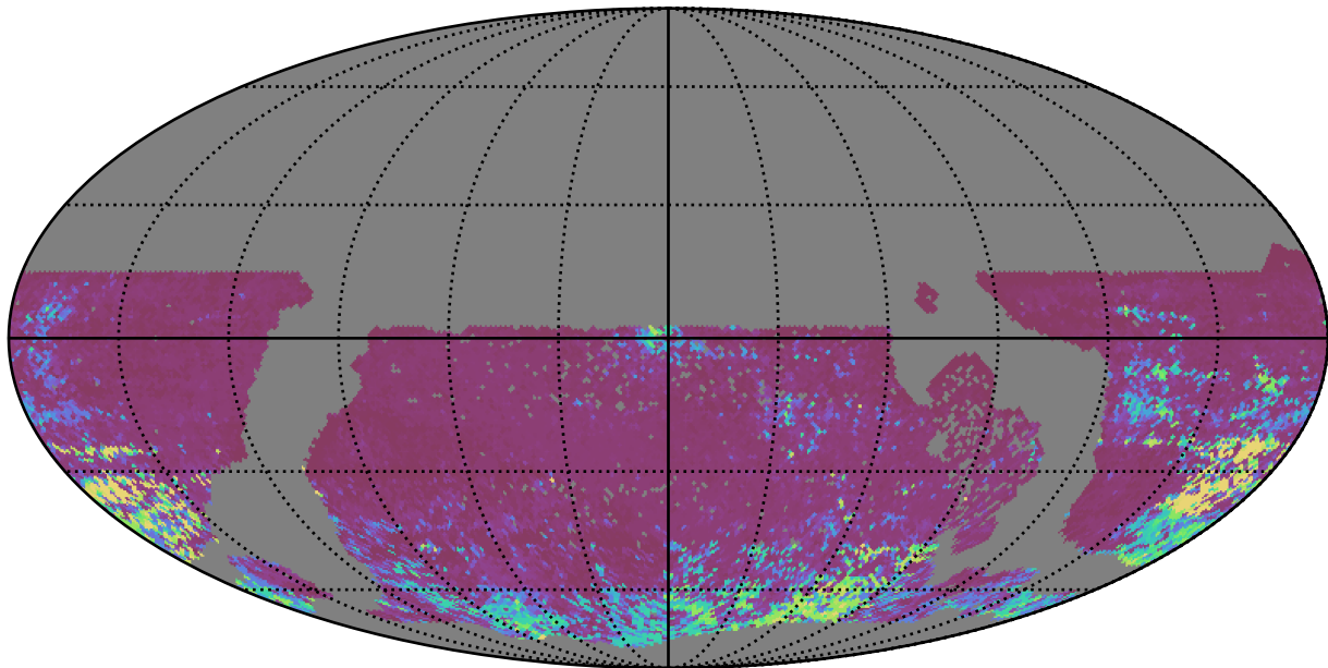
early_ss_template_fpextra3.0_v3.4_10yrs WFD i band: 75th Percentile Intranight Timespan
