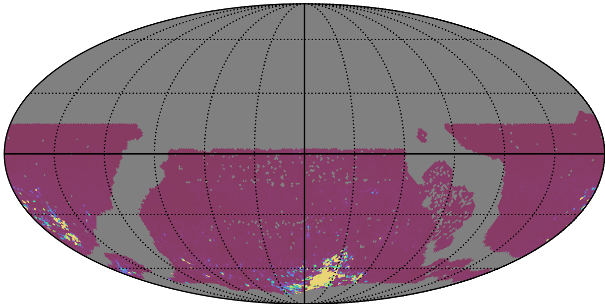
early_ss_template_fpextra3.0_v3.4_10yrs WFD gr bands: 75th Percentile Intranight Timespan
