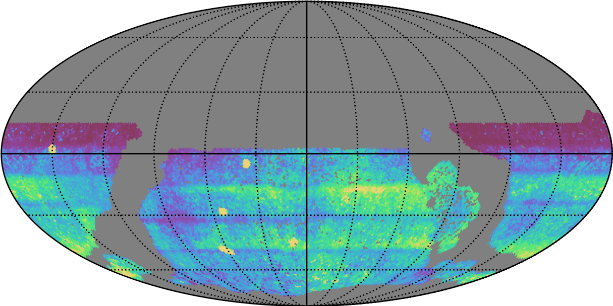
early_ss_template_fpextra3.0_v3.4_10yrs WFD all bands: 75th Percentile Intranight Timespan
