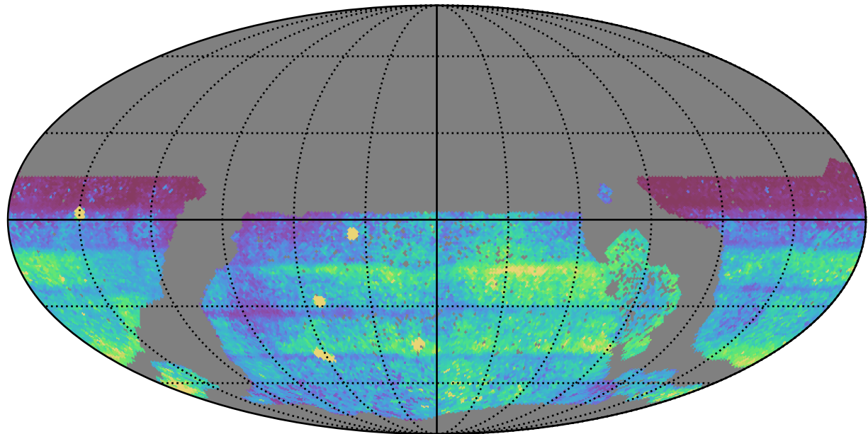
early_ss_template_fpextra3.0_v3.4_10yrs WFD: 75th Percentile Intranight Timespan
