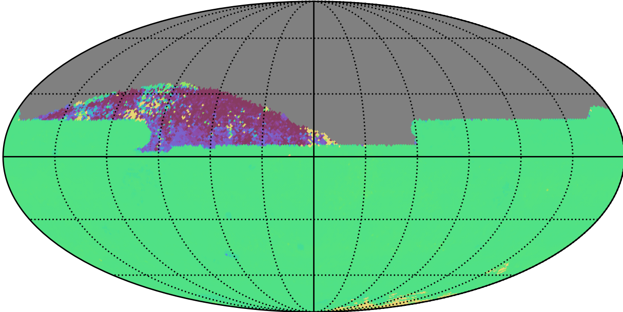
early_ss_template_fpextra3.0_v3.4_10yrs All sky zy bands: 75th Percentile Intranight Timespan
