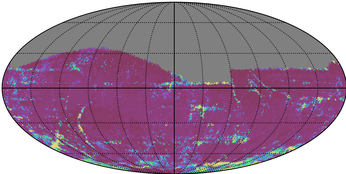
early_ss_template_fpextra3.0_v3.4_10yrs All sky z band: 75th Percentile Intranight Timespan
