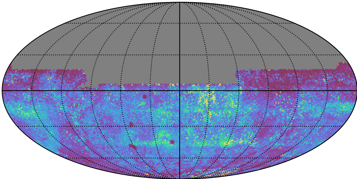
early_ss_template_fpextra3.0_v3.4_10yrs All sky y band: 75th Percentile Intranight Timespan
