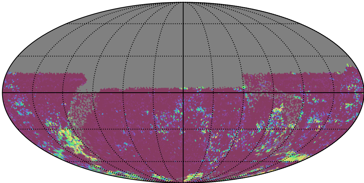
early_ss_template_fpextra3.0_v3.4_10yrs All sky u band: 75th Percentile Intranight Timespan
