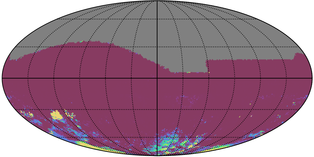
early_ss_template_fpextra3.0_v3.4_10yrs All sky ri bands: 75th Percentile Intranight Timespan
