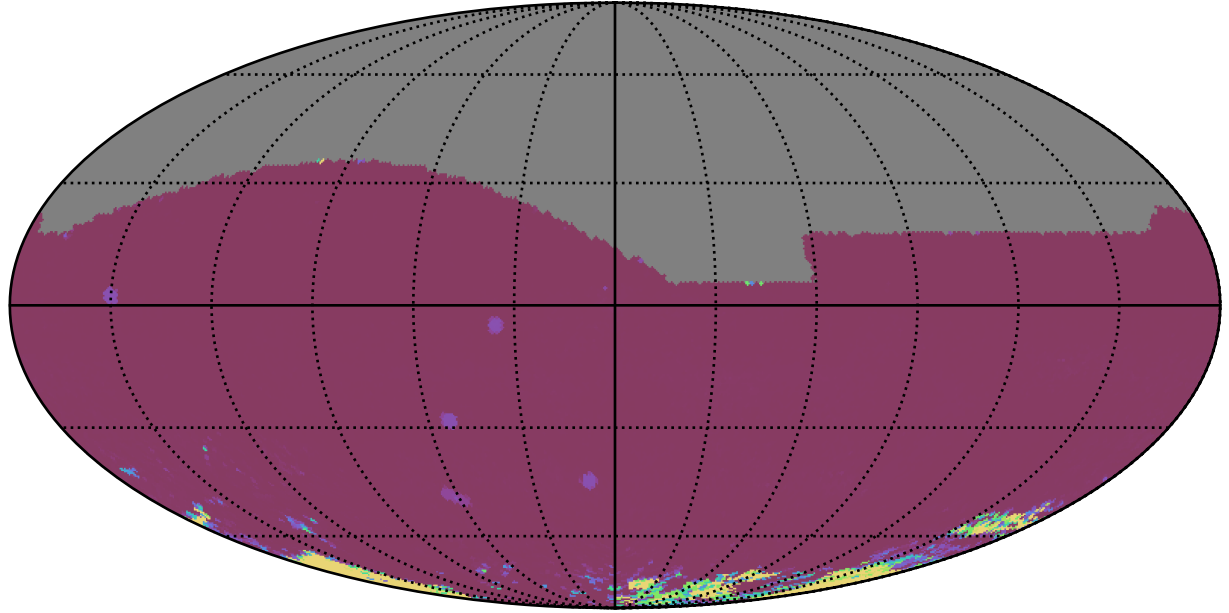
early_ss_template_fpextra3.0_v3.4_10yrs All sky iz bands: 75th Percentile Intranight Timespan
