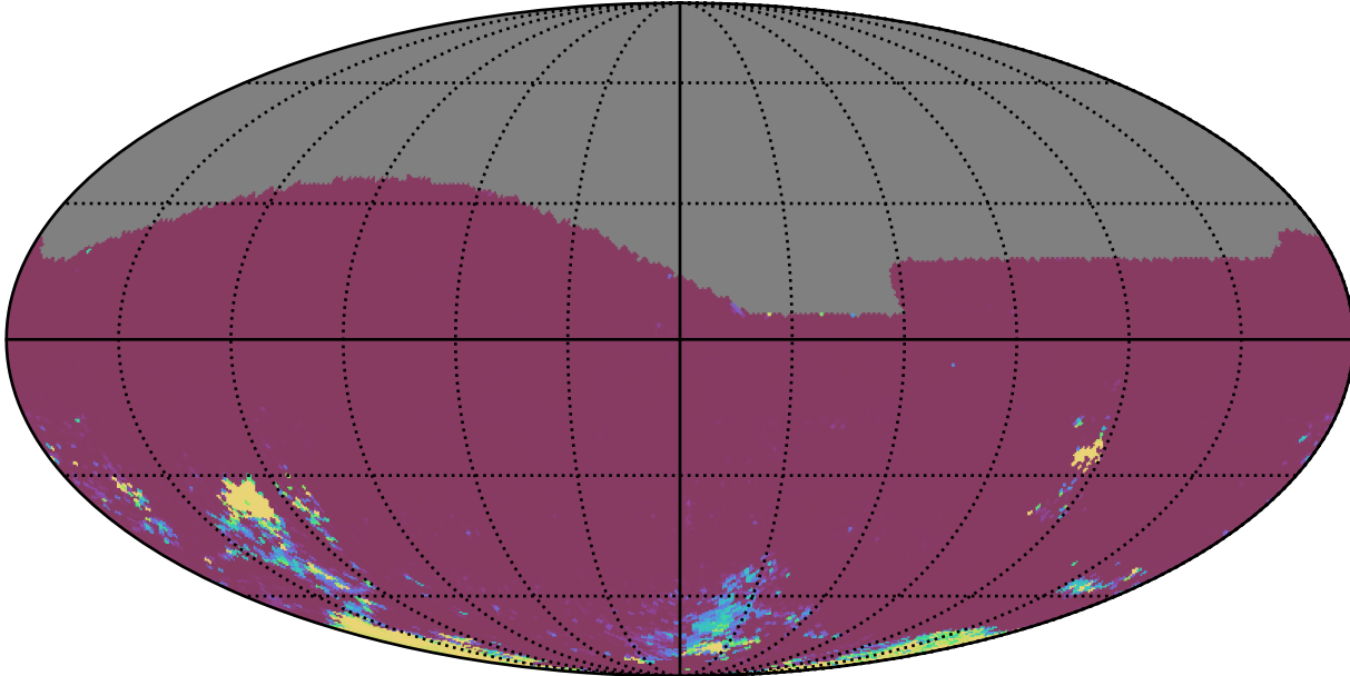
early_ss_template_fpextra3.0_v3.4_10yrs All sky gr bands: 75th Percentile Intranight Timespan
