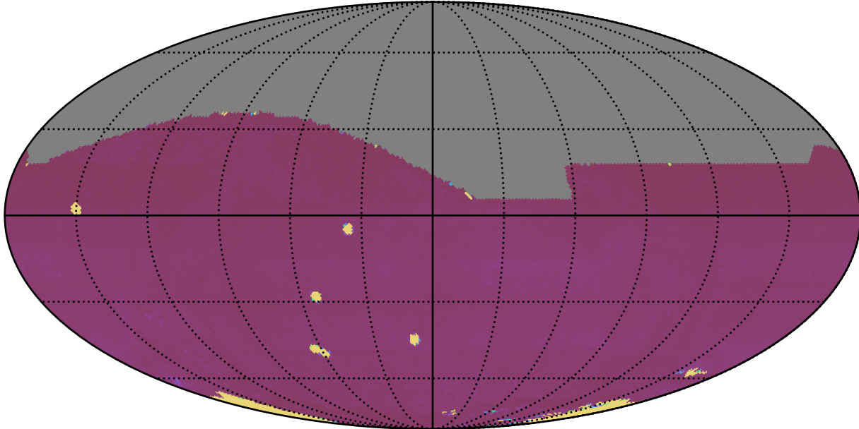
early_ss_template_fpextra3.0_v3.4_10yrs All sky all bands: 75th Percentile Intranight Timespan
