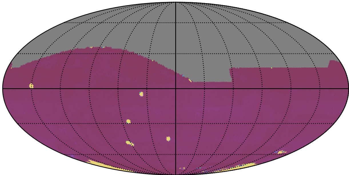
early_ss_template_fpextra3.0_v3.4_10yrs All sky: 75th Percentile Intranight Timespan
