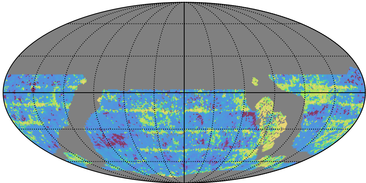
early_ss_template_fpextra3.0_v3.4_10yrs WFD z band: 20thPercentile Inter-Night Gap
