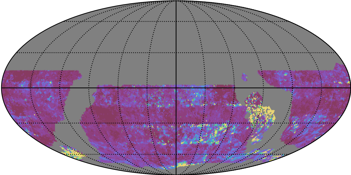
early_ss_template_fpextra3.0_v3.4_10yrs WFD u band: 20thPercentile Inter-Night Gap
