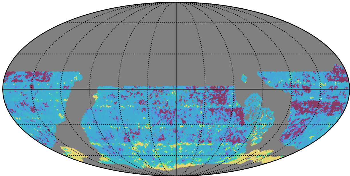
early_ss_template_fpextra3.0_v3.4_10yrs WFD r band: 20thPercentile Inter-Night Gap
