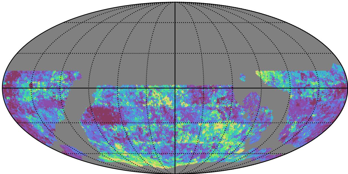
early_ss_template_fpextra3.0_v3.4_10yrs WFD g band: 20thPercentile Inter-Night Gap
