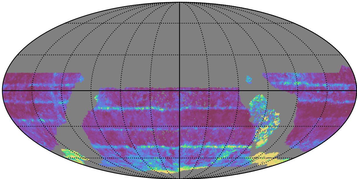
early_ss_template_fpextra3.0_v3.4_10yrs WFD all bands: 20thPercentile Inter-Night Gap
