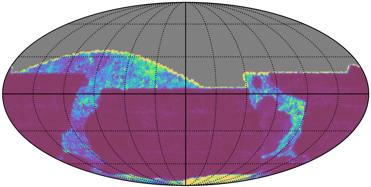
early_ss_template_fpextra3.0_v3.4_10yrs All sky z band: 20thPercentile Inter-Night Gap
