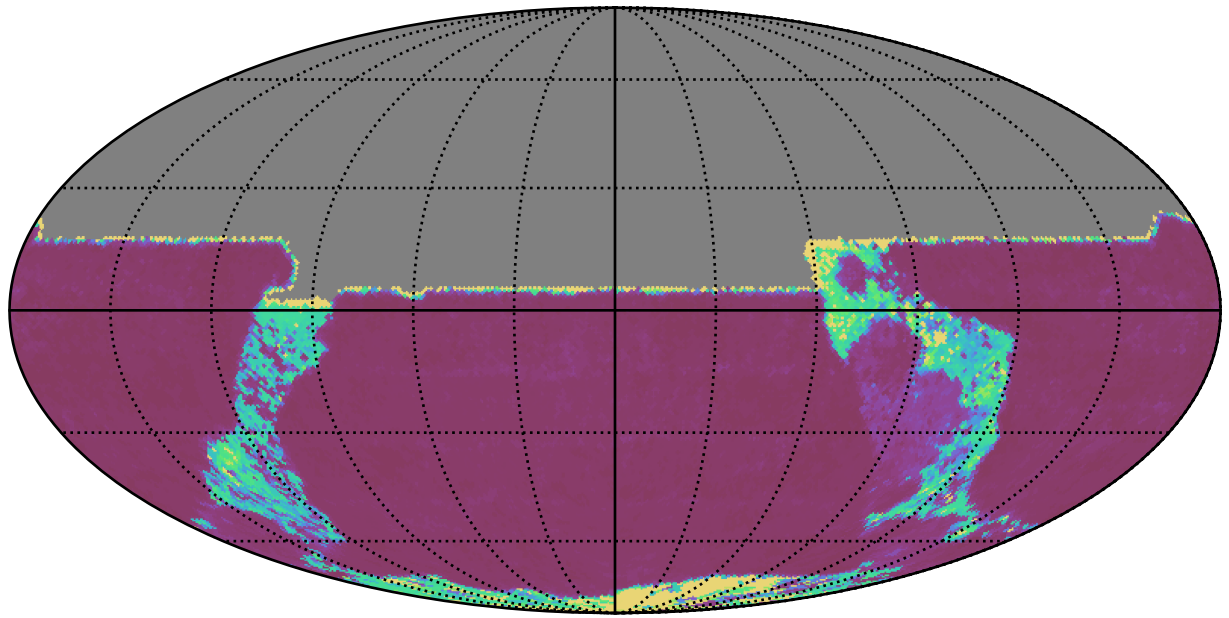
early_ss_template_fpextra3.0_v3.4_10yrs All sky y band: 20thPercentile Inter-Night Gap
