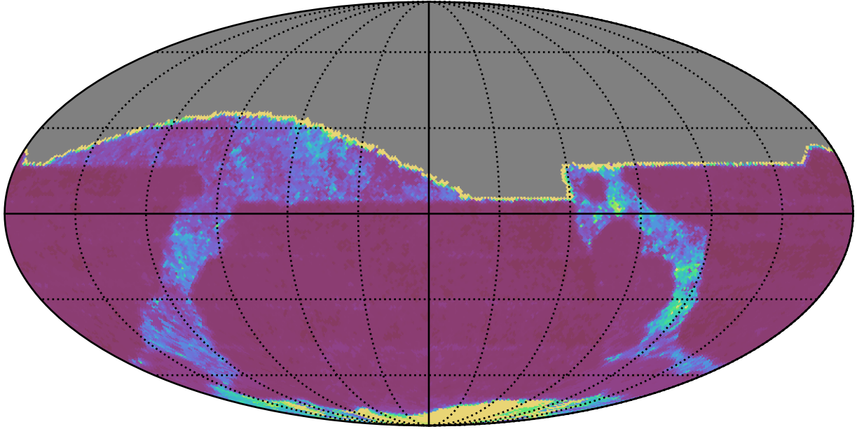
early_ss_template_fpextra3.0_v3.4_10yrs All sky r band: 20thPercentile Inter-Night Gap
