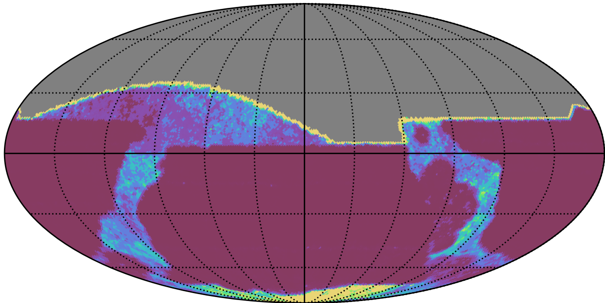
early_ss_template_fpextra3.0_v3.4_10yrs All sky all bands: 20thPercentile Inter-Night Gap
