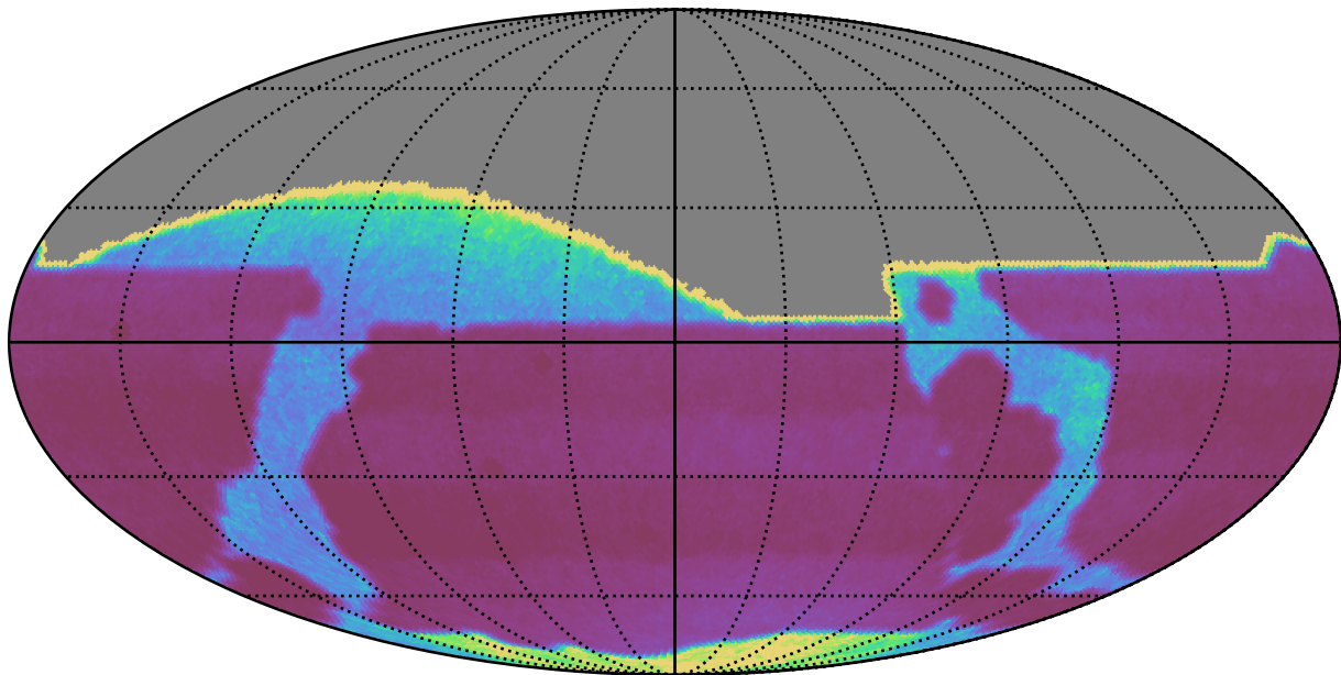
early_ss_template_fpextra3.0_v3.4_10yrs : properMotion
