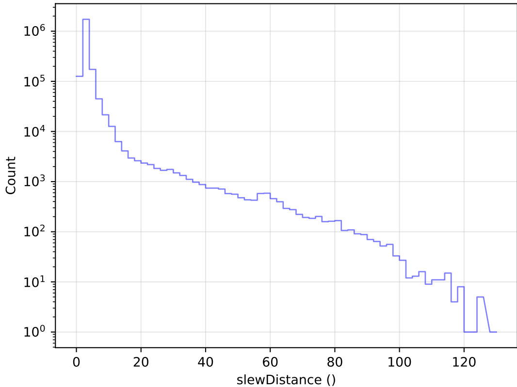
early_ss_template_fpextra3.0_v3.4_10yrs All visits: Slew Distance Histogram
