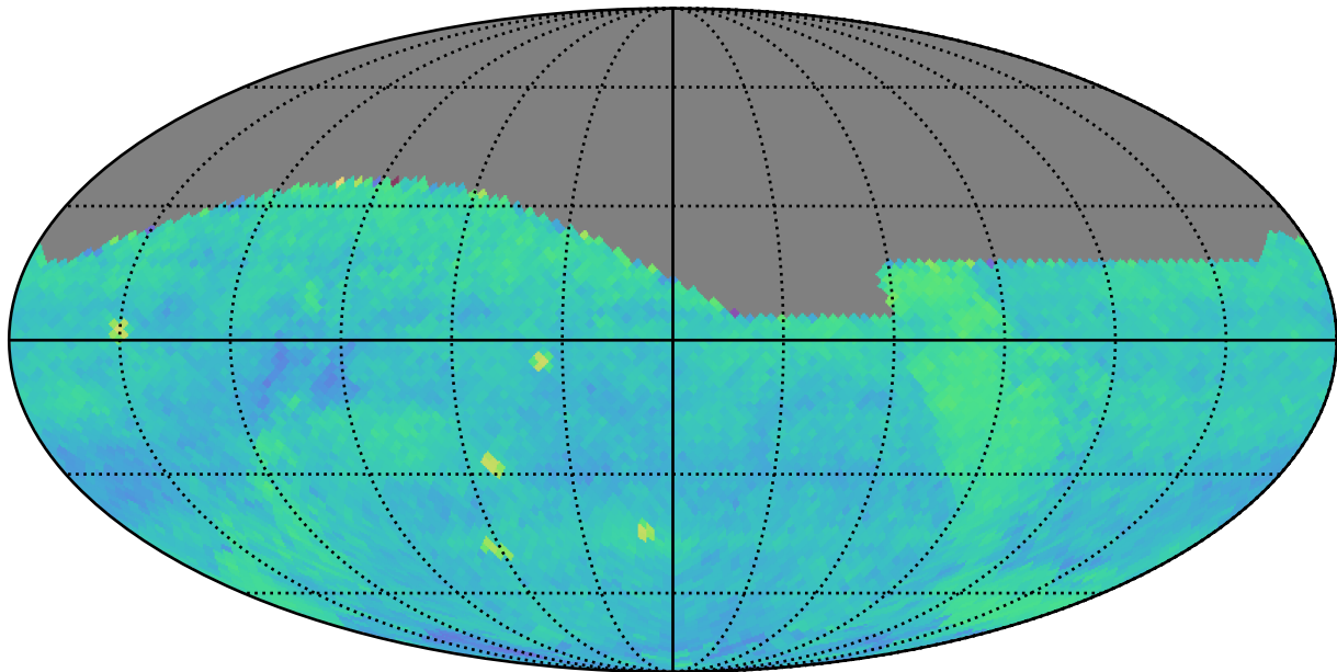
early_ss_template_fpextra3.0_v3.4_10yrs (g or r or i): PairFraction
